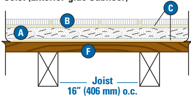
DensShield Tile Backer Over Conventional Joist (Exterior-glued Subfloor)
