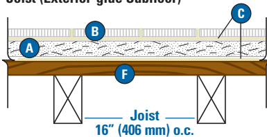
DensShield Tile Backer Over Conventional Joist (Exterior-glued Subfloor)
